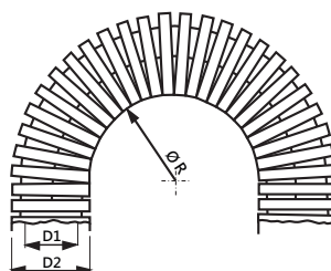
DIMENSION DRAWING &amp; TECHNICAL DETAILS
