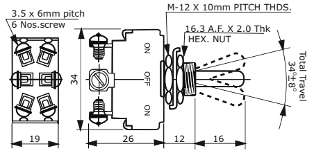
DOUBLE POLE UNSEALED
