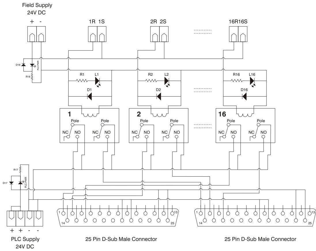
Connection Diagram of TT-IMRB-16024D2S-DI2X25M
