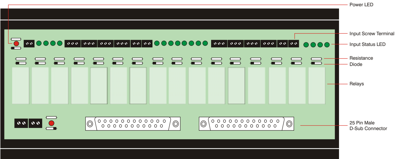
Layout of TT-IMRB-16024D2S-DI2X25M
