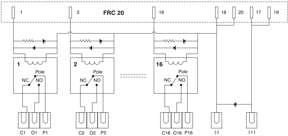
Connection Diagram of TT-IMRB-16024D1S-DO(F20)
