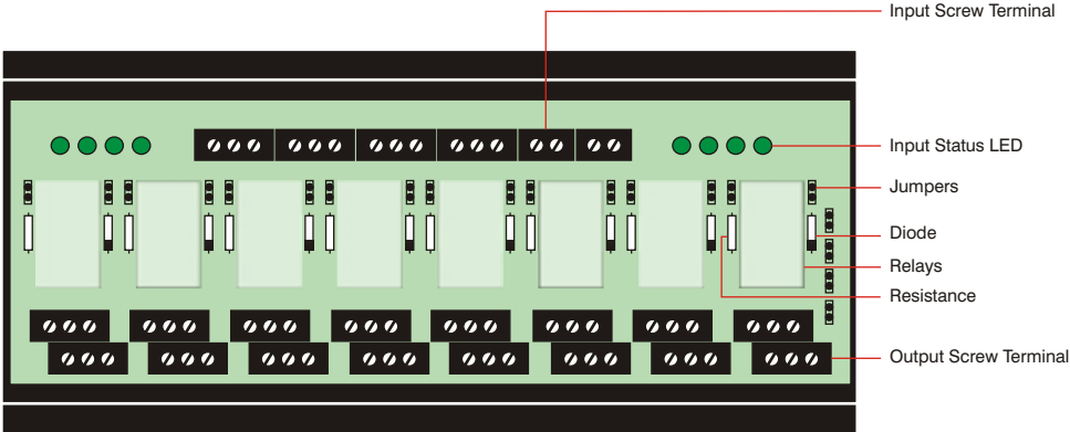
Layout of TT-IMRB-08024D2S-C
