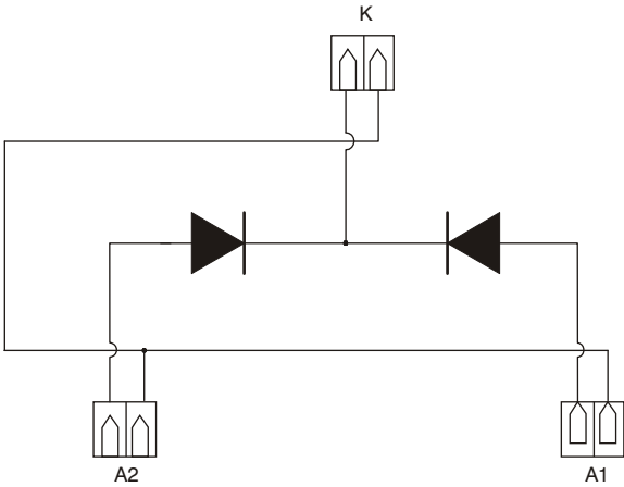
Connection Diagram of TT-IMPB-Diode Module (10A)
